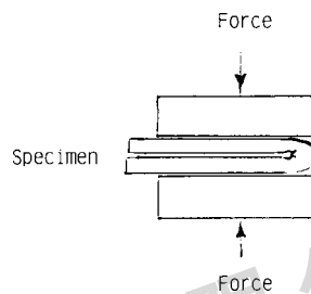
FIG. 14 Bend and Flatten
